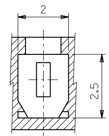
SECT. W-W (SCALE 10:1)
