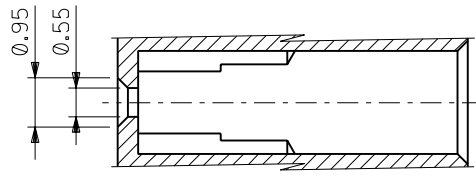
SECT. X-X (SCALE 10:1)
