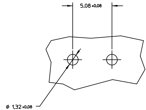
PRINTED CIRCUIT BOARD HOLE PATTERN
