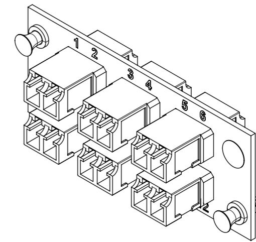
ISO VIEW
