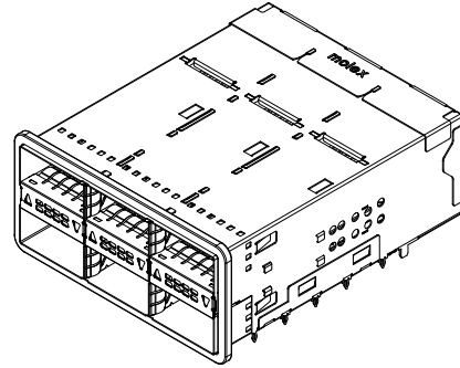
171262 - 2X3 CONNECTOR WITH ELASTOMERIC EMI GASKET
