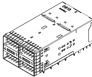
171722 - 2X1, 2X2 & 2X3 CONNECTORS WITH METAL EMI GASKET & ENHANCED EMI CAGE CONSTRUCTION
