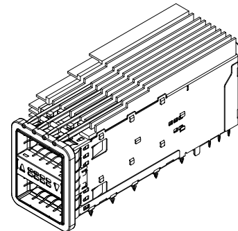
171722 - 2X1, 2X2 & 2X3 CONNECTORS WITH METAL EMI GASKET & ENHANCED EMI CAGE CONSTRUCTION
