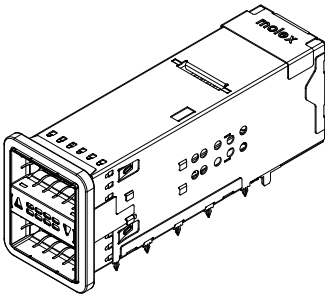
171208 - 2X1 CONNECTOR WITH ELASTOMERIC EMI GASKET
