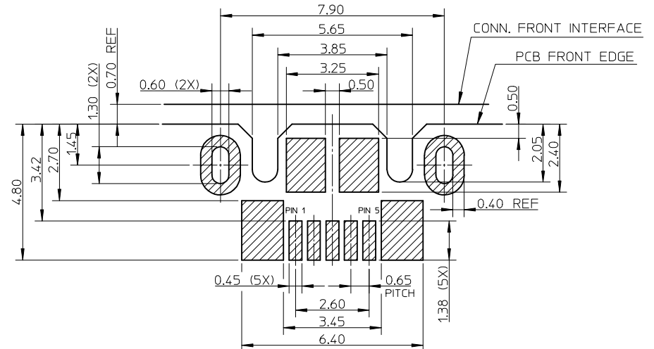
RECOMMENDED P.C.B. PATTERN LAYOUT GENERAL TOLERANCE : ±0.05MM
