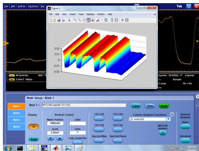
Custom analysis - Waterfall display generated from oscilloscope data using MATLAB.
