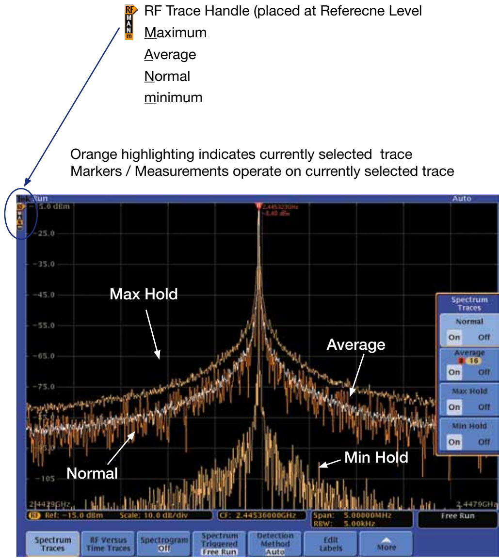
Figure 13. Spectrum Traces.
