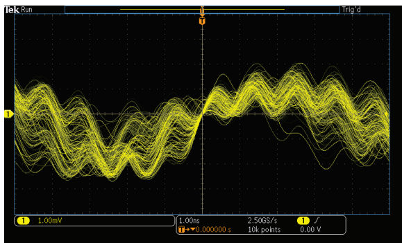
Figure 13: High-frequency noise riding on critical signal.
