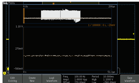
Figure 21: Noise-free CAN signal generated by the ARB.
