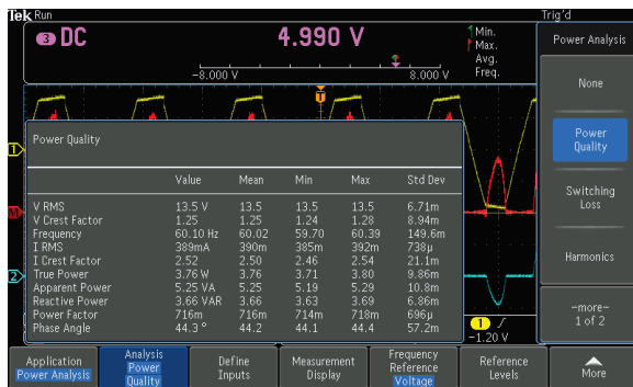
Figure 28: Power Supply input power quality measurements.
