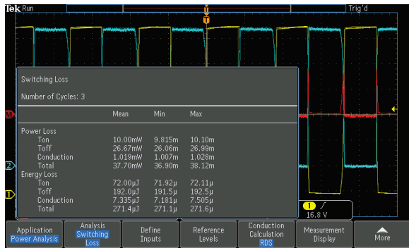
Figure 31: Switching Loss measurements.
