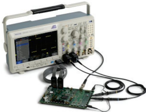
Figure 18: Using the integrated arbitrary / function generator as a source.
