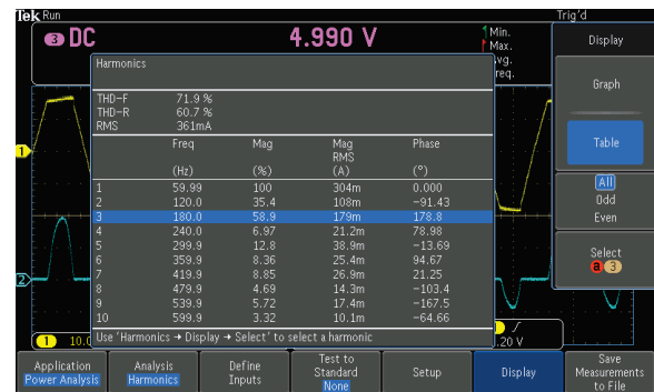
Figure 30: Tabular display of input current harmonics.
