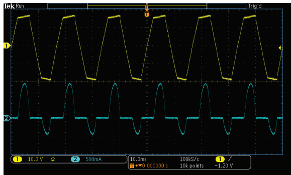
Figure 25: AC input voltage (yellow) and current (blue) waveforms.
