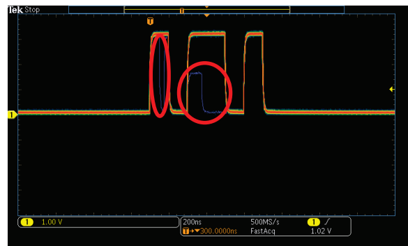
Figure 3: FastAcq capture of signal anomalies
