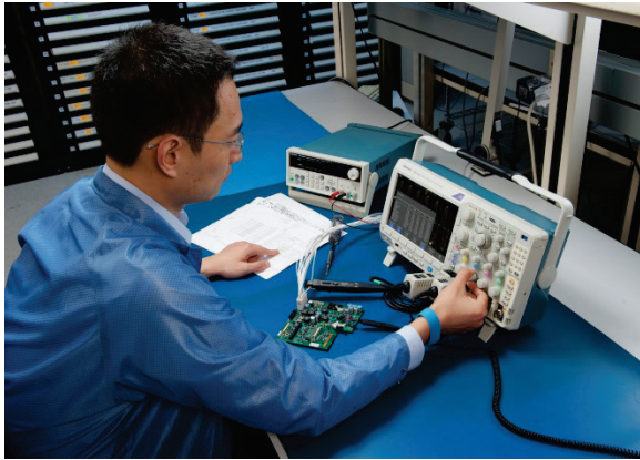
Figure 24: MDO3000 with differential voltage probe and current probe.
