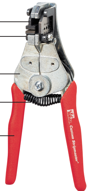
Die-type blades incorporate a counterbored hole sized to the insulation and an inner cutting hole sized to the conductor. This varies depending on insulation type and thickness.
