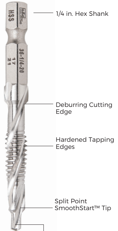
3-flute Design
