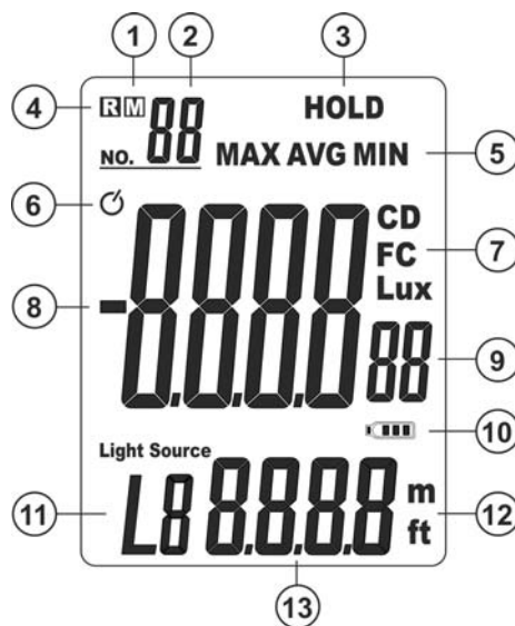
Fig. 2: Display description
