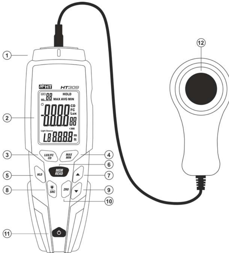
Fig. 1: Instrument description
