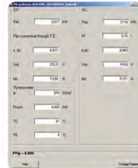
PV plant performance outcome on PC
