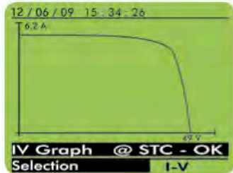
I-V curve
