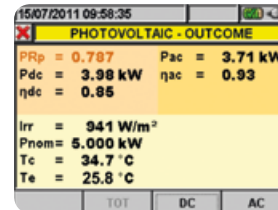
PV plant performance outcome on instrument display
