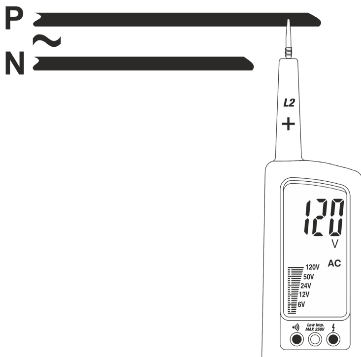
Fig. 5: 1-wire AC Voltage detection
