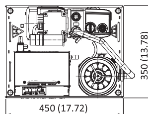
T-Station 300 Wet with E2M1.5 backing pump
