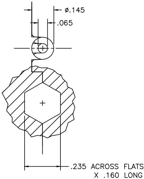
GAGING DIMENSIONS
