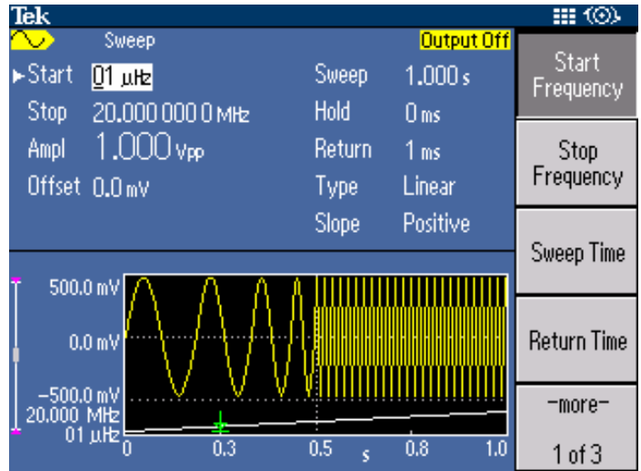
Frequency range from 1 \mu Hz to 20 MHz, supports a wide range of amplifier and filter testing applications.
