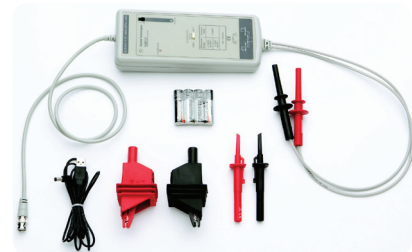
N2891A 70 MHz high voltage differential probe
