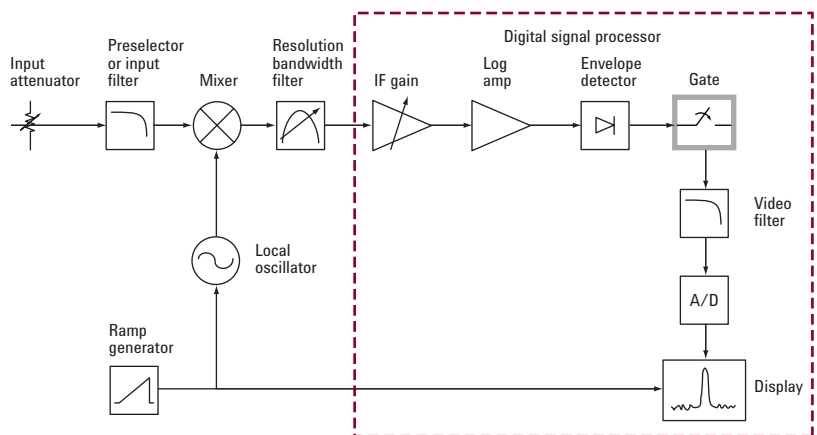
Figure 23. Spectrum analyzer block diagram with gated video time-gating
