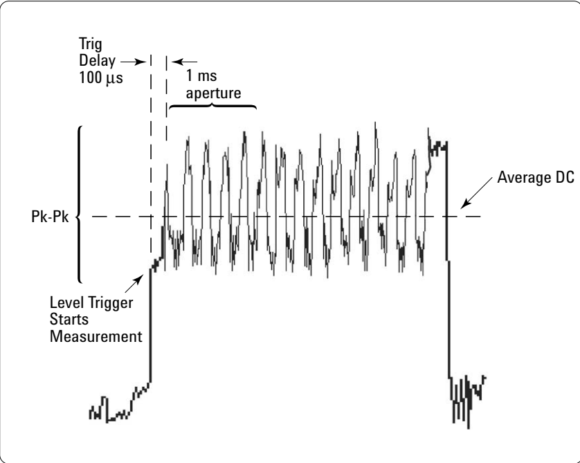
Figure 2. Peak detect occurs at 20-μs intervals over the duration of the measurement aperture
