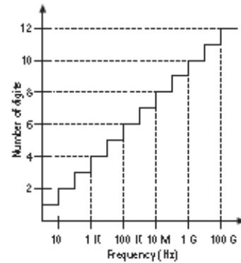
Figure 2. The number of digits displayed by a direct counter vs. frequency (for a 1 second gate time)
