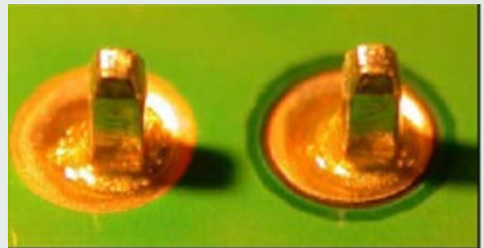
Figure 4: High-solids flux residue around a through-hole component. [1]
